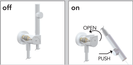
HYDROSCOPINO CON EROGAZIONE UNICA SUPERIORE TIPO LASER HYDROBRUSH WITH ONLY SPRAYER UP LIKE LASER ART. 0403/ID/LA, 0903/ID/LA, 0303/ID/LA
