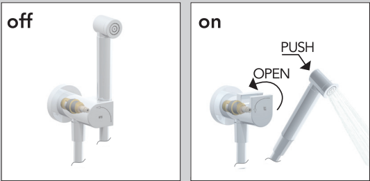
HYDROSCOPINO CON EROGAZIONE UNICA TIPO DOCCETTA HYDROBRUSH WITH ONLY SPRAYER LIKE HANDSHOWER ART. 0403/ID, 0903/ID, 7503/ID, 3303/ID, 0303/ID, 1403/ID, 4503/ID
